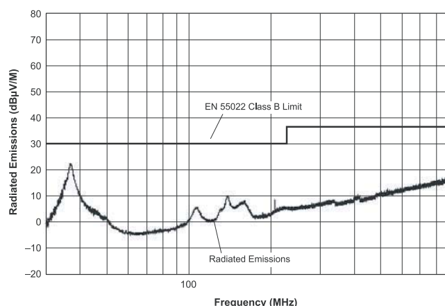
UWP-15/200-D5 Radiated Emissions EN 55022 Class B, 10 Meters Converter Output = +15Vdc @ +180mA
