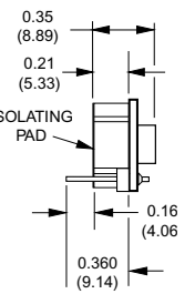
Case B5A Horizontal Mounting
