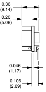
Case B5B Reverse Pin Vertical Mounting (Tyco-compatible)
