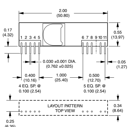
Case B5 Vertical Mounting (Standard)
