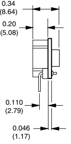
Case B5 Vertical Mounting (Standard)
