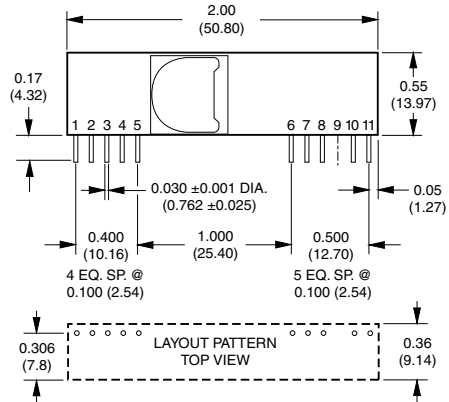
Case B5B Reverse Pin Vertical Mounting (Tyco-compatible)
