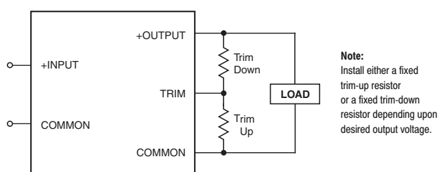
Figure 7. Trim Connections Using Fixed Resistors
