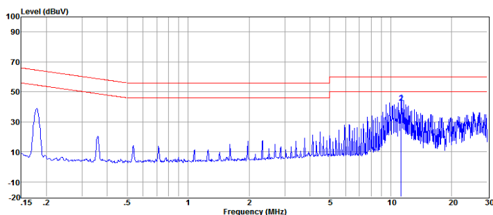
Graph1. Conducted Emissions Performance, Positive Line, CISPR 22, Class B, Full load
