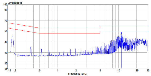
Graph1. Conducted Emissions Performance, Negative Line, CISPR 22, Class B, Full load
