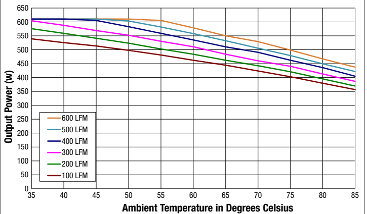
Figure 5. Maximum Power Temperature Derating with Baseplate (Vin=48V, airflow is from Vin- to Vin+ on 10x10 inch PCB)
