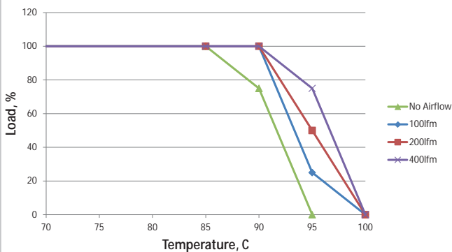
MTC1S1205MC - 18Vin
