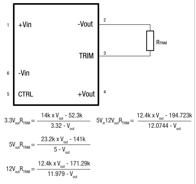
Figure 2. Trim connections to increase the output voltage
