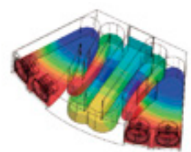
Acoustic Waves
