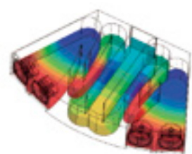
Acoustic Waves
