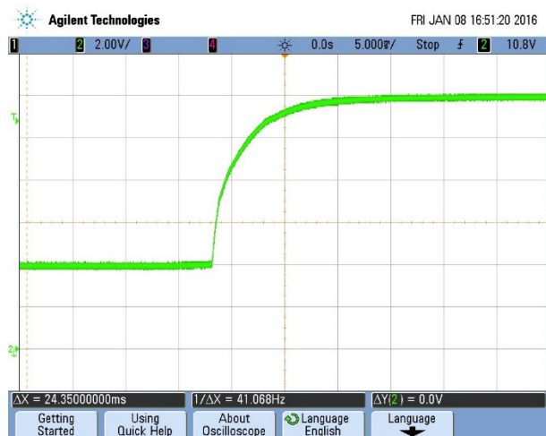
Start-up into a Pre-bias Load@25°C
