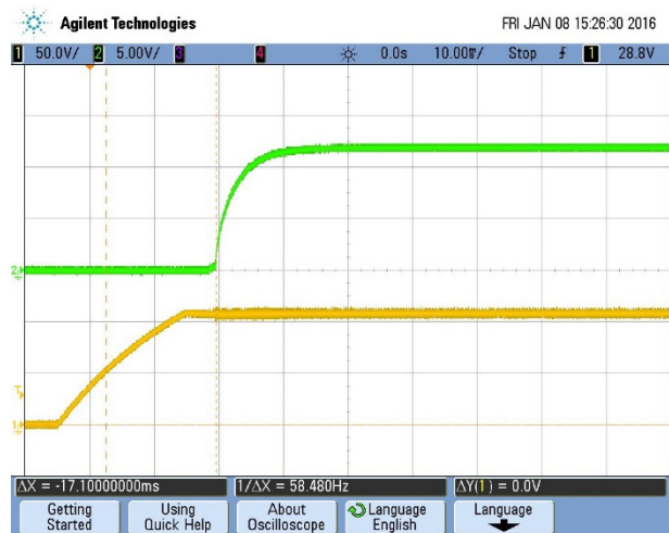
Turn-on transient at zero load current (10 mS/div, Top Trace: Vout, 5V/div; Bottom Trace: Vin, 50V/div)
