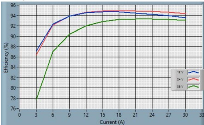
Fig. 4: ICH0130V1PC Efficiency Curve
