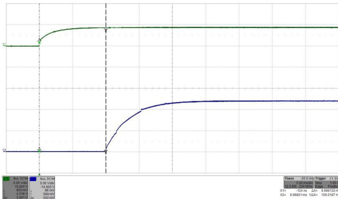
Fig. 16: Turn-on by ON/OFF transient (with Vin applied) at full rated load current (resistive) at Vin = 24V. Top trace (C1): ON/OFF signal (5 V/div.). Bottom trace (C4): Output voltage (5 V/div.). Time: 5 ms/div.
