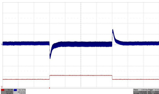
Fig. 18: Output voltage response to load current step change 50% - 75% - 50% (15A-22.5A-15A) with di/dt = 1A/μs at Vin = 24V. Top trace (C4): Output voltage (200 mV/div.). Bottom trace (C3): Load current (20A/div.). Co = 470 μF/70mΩ. Time: 1ms/div.
