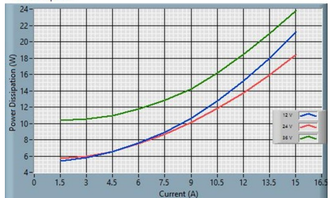
Fig. 7: ICH0415V1PC Power Dissipation
