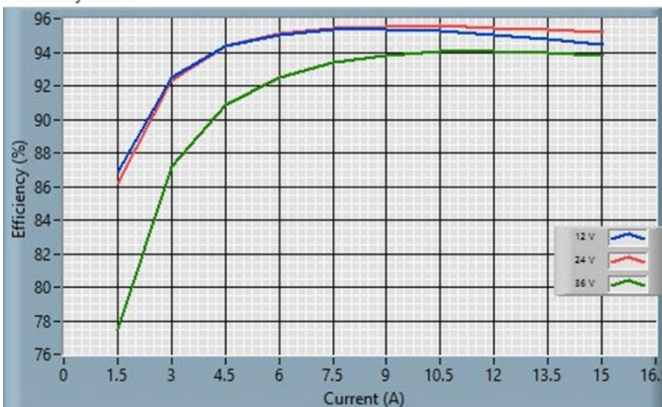
Fig. 6: ICH0415V1PC Efficiency Curve
