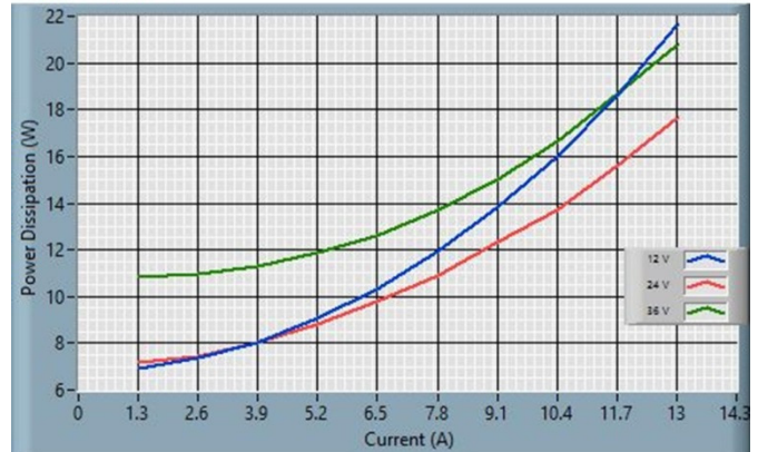
Fig. 9: ICH0513V1PC Power Dissipation
