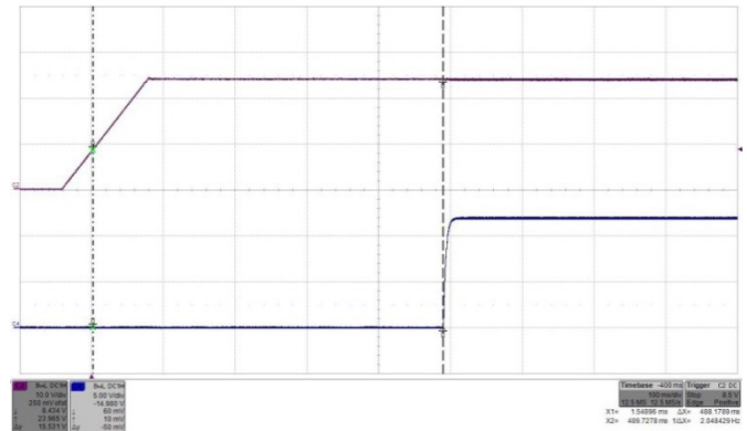
Fig. 17: Turn-on by Vin (ON/OFF high) transient at full rated load current (resistive) at Vin = 24V. Top trace (C2): Input voltage Vin (10 V/div.). Bottom trace (C4): Output voltage (5 V/div.). Time: 100 ms/div.
