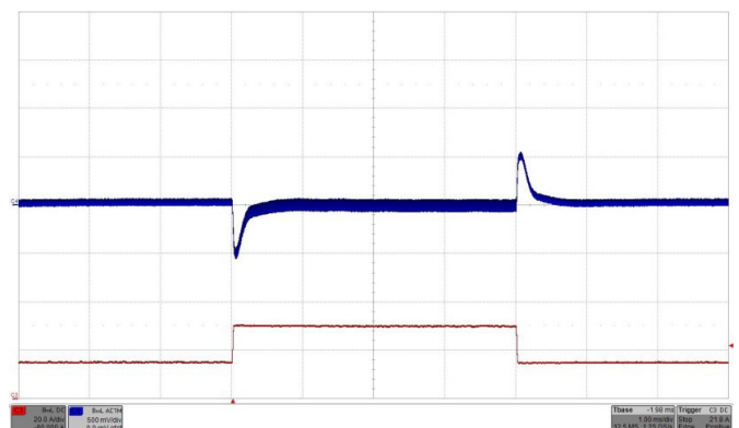
Fig. 19: Output voltage response to load current step change 50% - 100% - 50% (15A-30A-15A) with di/dt = 1A/μs at Vin = 24V. Top trace (C4): Output voltage (500 mV/div.). Bottom trace (C3): Load current (20A/div.). Co = 470 μF/70mΩ. Time: 1ms/div.
