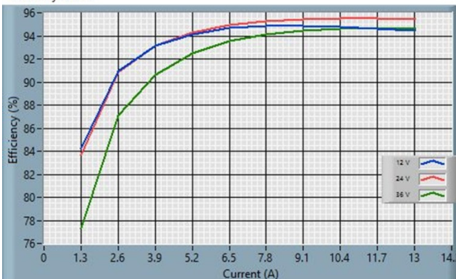
Fig. 8: ICH0513V1PC Efficiency Curve
