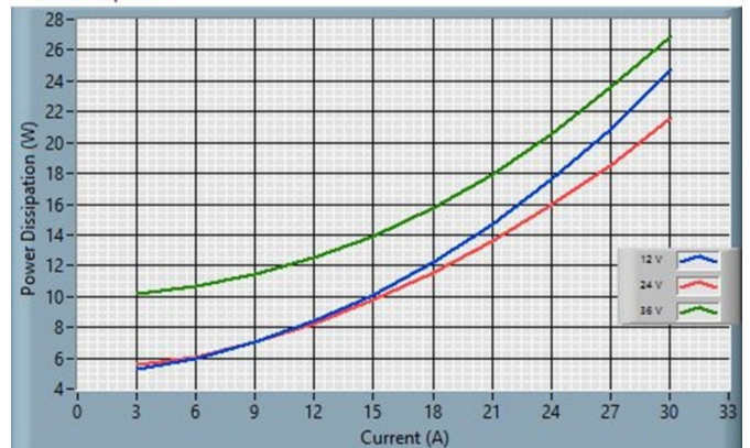
Fig. 5: ICH0130V1PC Power Dissipation
