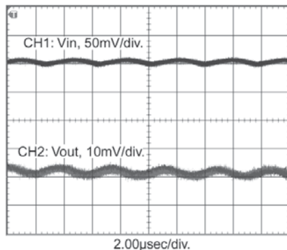
7805SR-C V_{IN} = 12\text{V} , I_{LOAD} = 50\text{mA}
