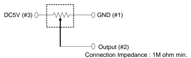
Fig.6 Circuit Diagram
