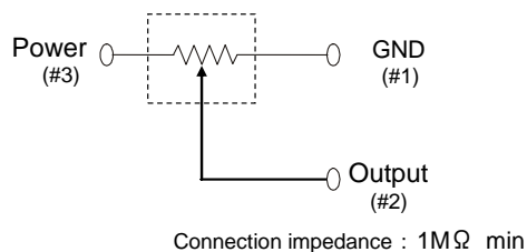
Fig.3 Circuit Diagram
