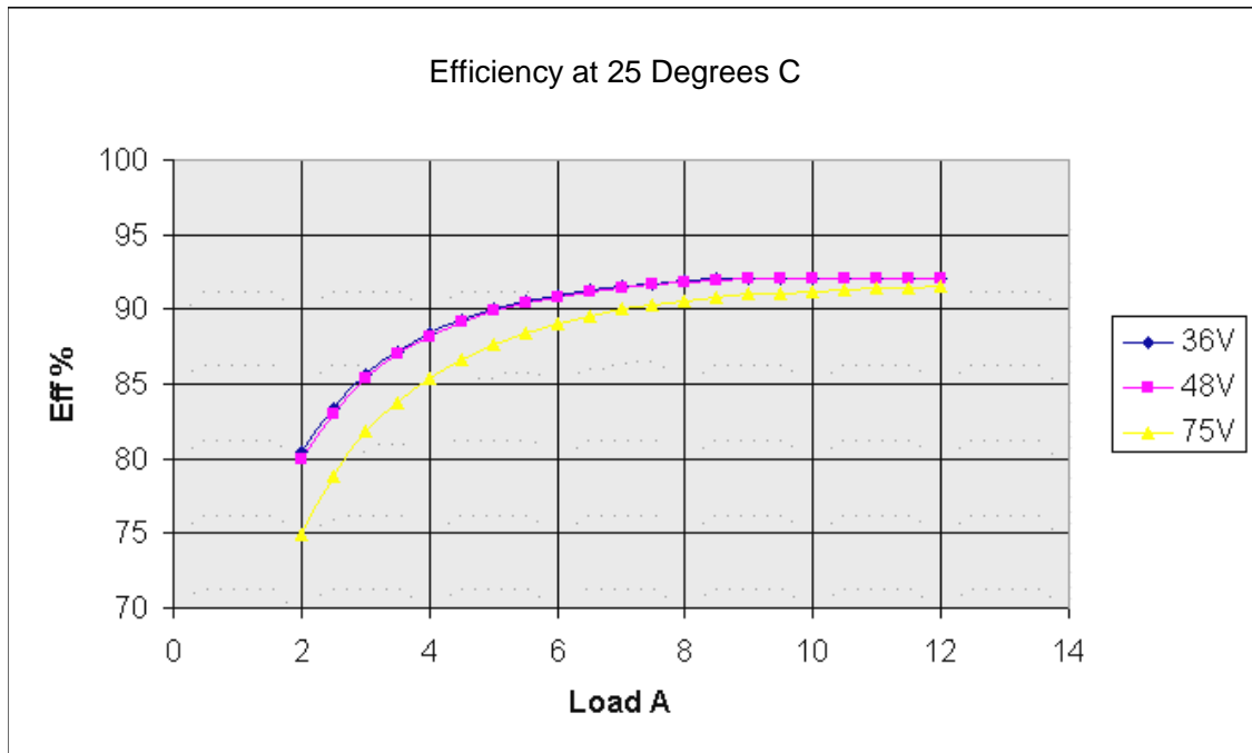
Figure 6 QHS12-120 Efficiency
