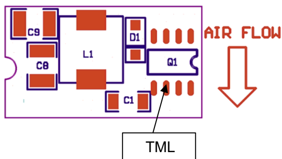
Figure 1. Thermal Tests Set-Up
