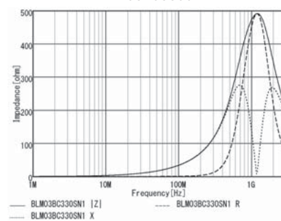
BLM03BC330SN1
