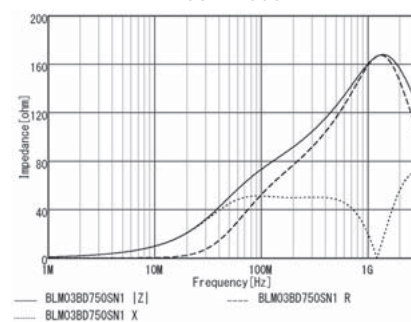
BLM03BD750SN1
