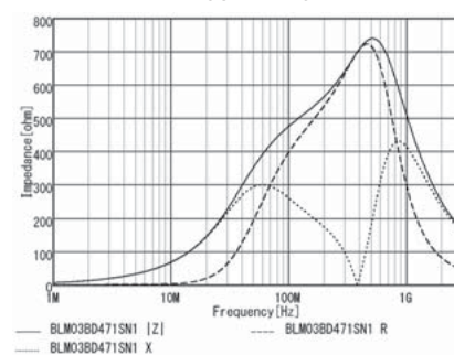
BLM03BD471SN1
