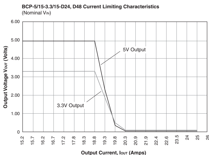
Figure 2. Current Limiting Characteristics
