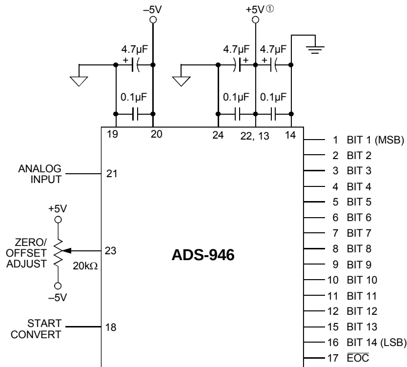
Figure 3. Typical ADS-946 Connection Diagram
