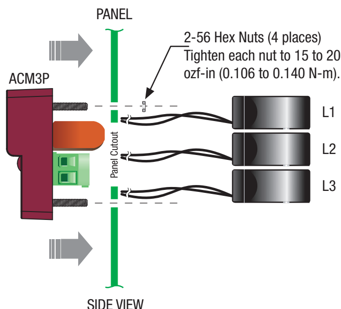
Figure 1. Panel Installation
