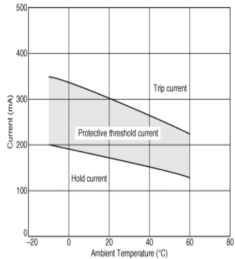
Protective Threshold Current Range
