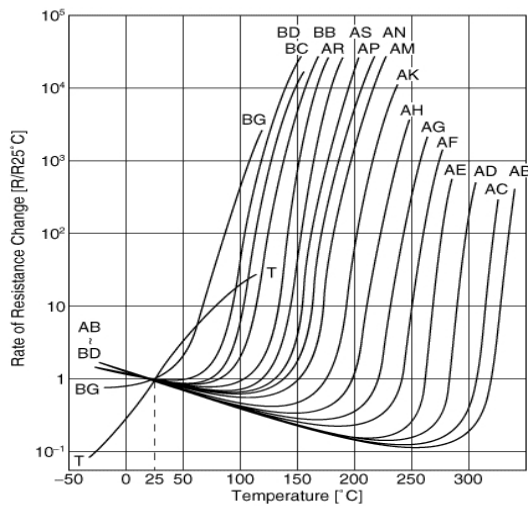
Resistance-Temperature Charac.
