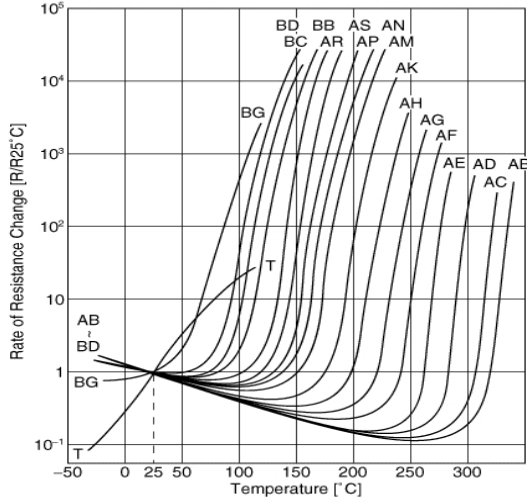
Resistance-Temperature Charac.
