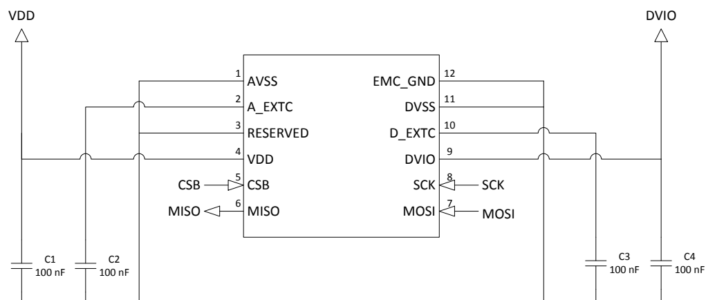
Figure 15 Application schematic
