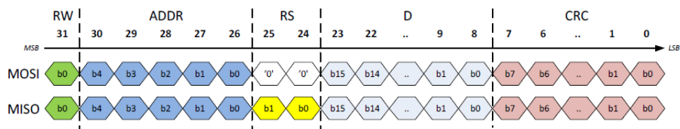
Figure 13 SPI Frame
