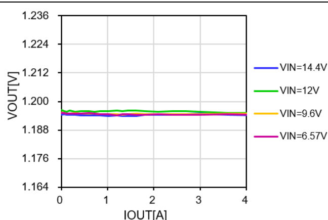
Figure 18. VOUT vs. Load Current and Line Voltage @+25°C (VOUT=1.2V)
