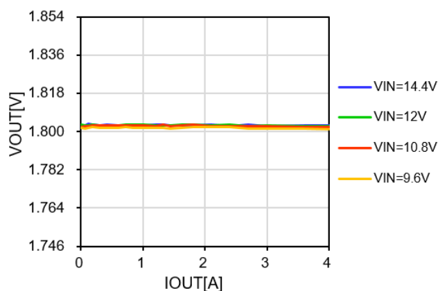
Figure 12. Vo vs. Load Current and Line Voltage @+25°C (VOUT=1.8V)
