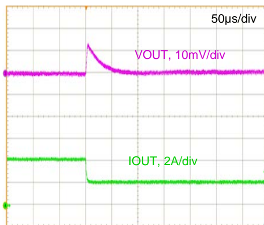
Figure 28. Step Load Transient Response (VIN=12V, VOUT=0.7V, COUT=200μF, IOUT=4 to 2A, 1.0A/μs)
