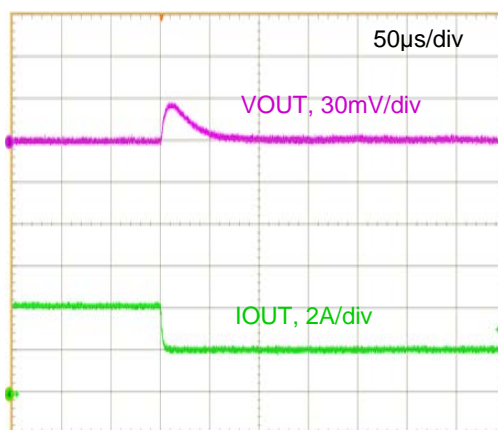
Figure 16. Step Load Transient Response (VIN=12V, VOUT=1.8V, COUT=200μF, IOUT=4 to 2A, 1.0A/μs)
