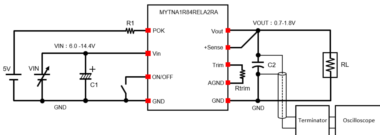
Figure 29. Test Circuit
