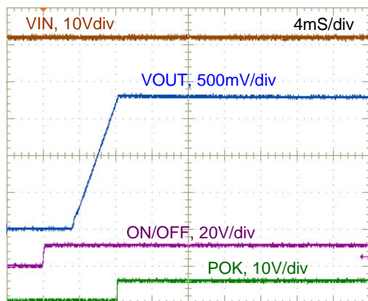
Figure 13. On/Off Enable wave form @+25°C (VIN=12V, VOUT=1.8V, IOUT=4A)
