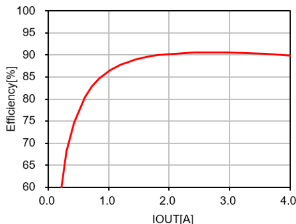
Figure 1. Efficiency Plot
