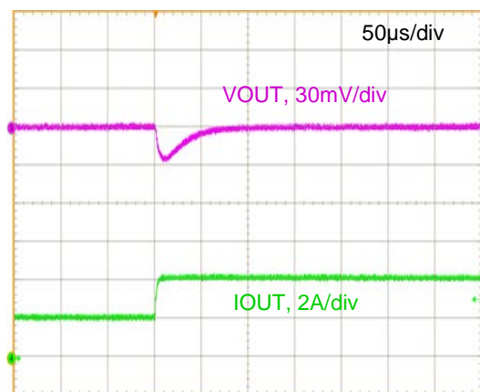
Figure 15. Step Load Transient Response (VIN=12V, VOUT=1.8V, COUT=200μF, IOUT=2 to 4A, 1.0A/μs)
