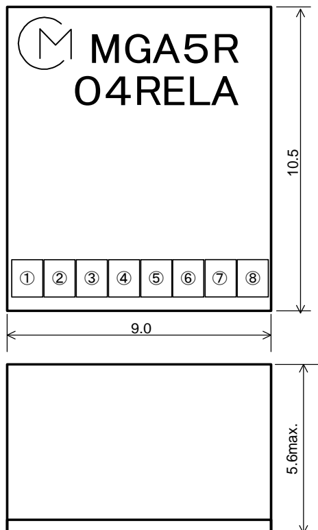
< Top View >
