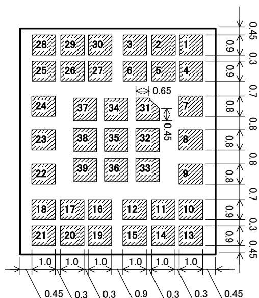
< Bottom View >
