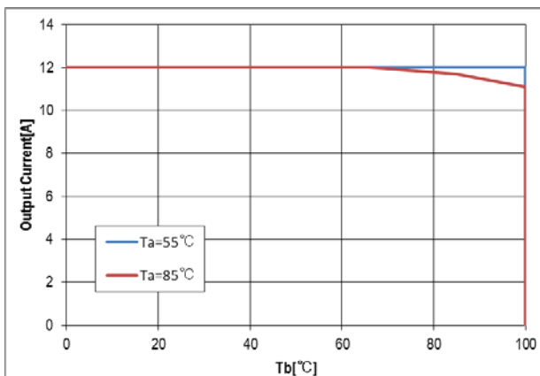
Thermal Derating (conduction cooling) ( V_{in}=48\text{V} , See Technical Notes)
