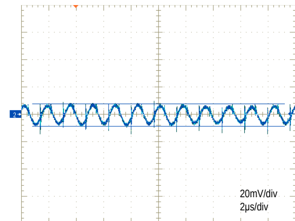
Output Ripple and Noise ( V_{in}=48\text{V} , V_{out}=5\text{V} , I_{out}=12\text{A} , T_a=+25^{\circ}\text{C} )
