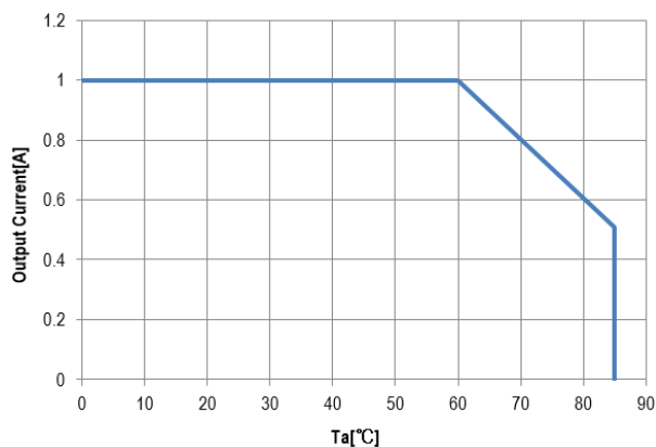
Thermal Derating Unit under test (UUT) is covered by acrylic box to avoid airflow. (V in =48V, See Technical Notes)
