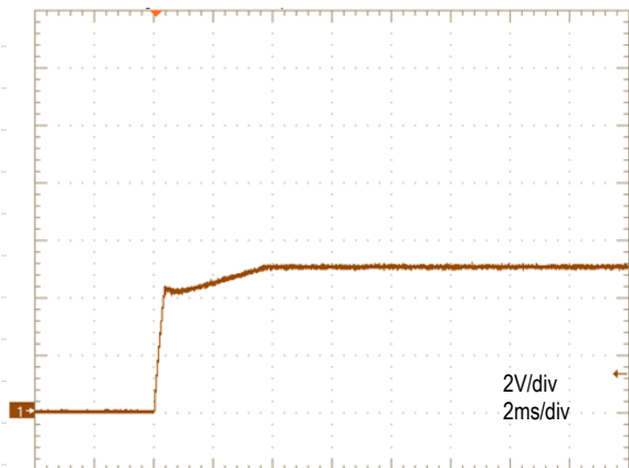
Vout Start-up (Vin=48V, Iout=2A, Ta=+25°C)
