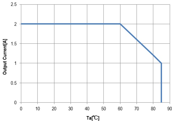
Thermal Derating Unit under test (UUT) is covered by acrylic box to avoid airflow. (Vin=48V, See Technical Notes)
