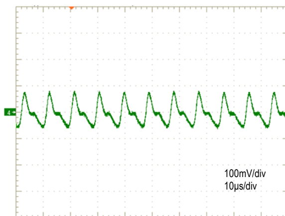
Output Ripple and Noise (Vin=48V, Iout=2A, Ta=+25°C)
