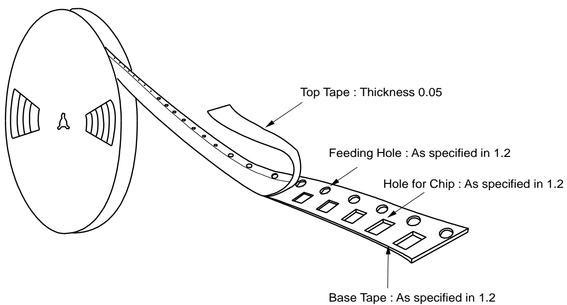
Fig3 Taping Diagram
