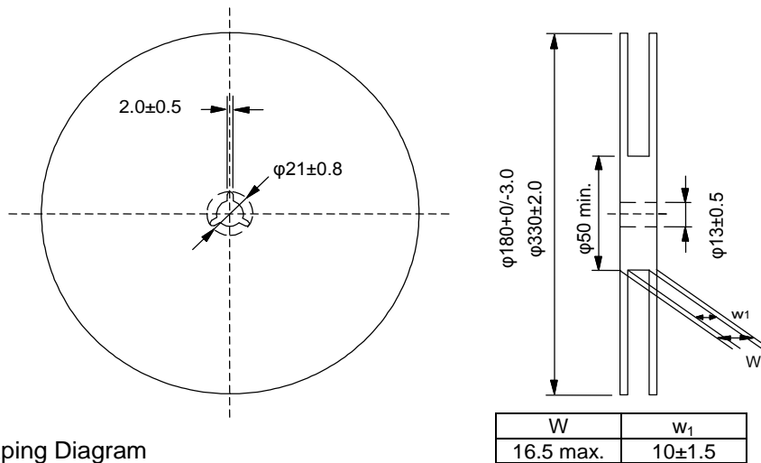
Fig.2 Dimensions of Reel
