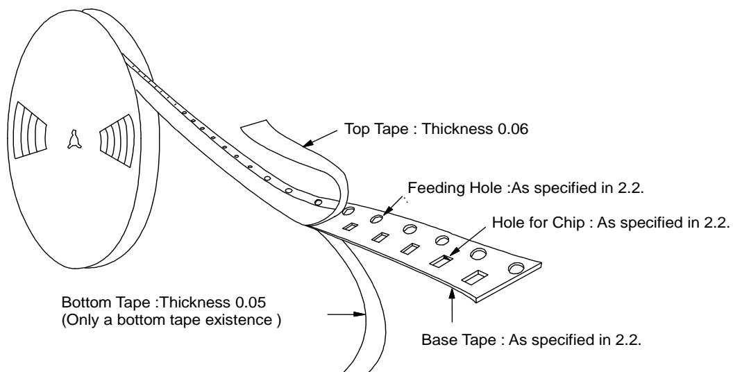
Fig.3 Taping Diagram
