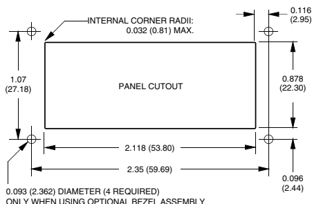
RECOMMENDED DRILL AND PANEL CUTOUT DIMENSIONS
