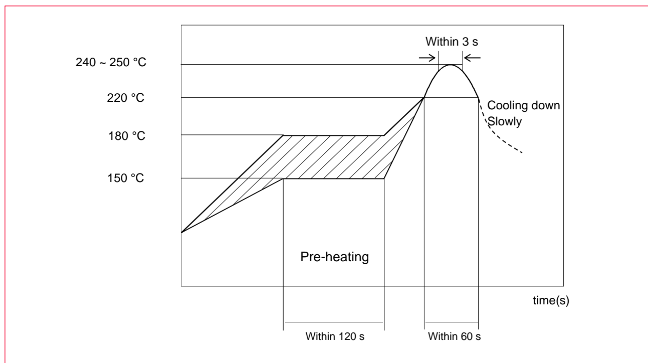
Figure 8: Reflow Soldering Standard Conditions (Example)
