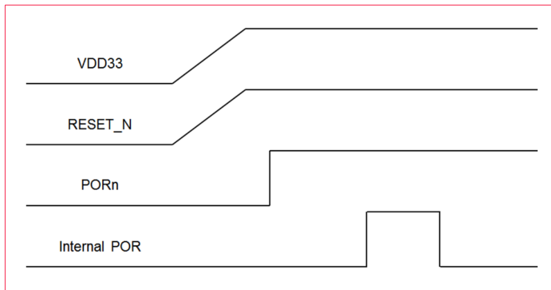
Figure 5: Power-On Sequence
