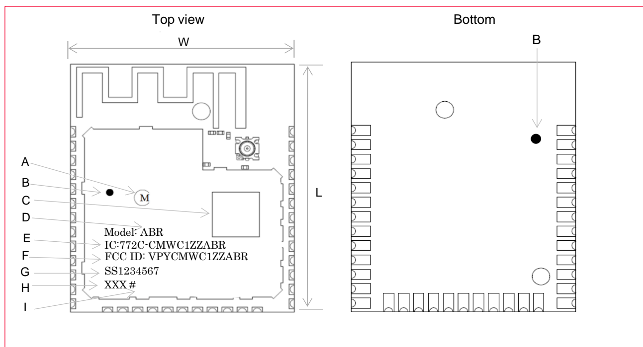
Figure 2: Construction, Dimensions, Marking and Terminal Configurations
