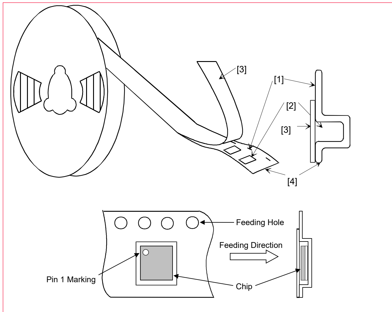
Figure 21: Taping Diagrams
