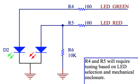
<Common cathode diagram>
