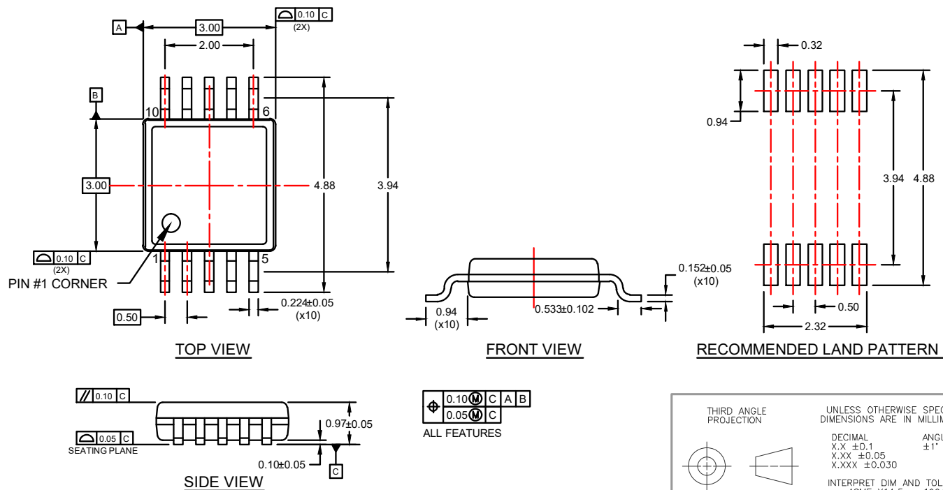
Figure 46. Package Drawing 10-lead MSOP 3 × 3 × 0.86 mm
