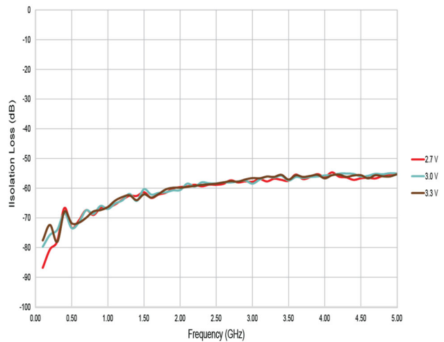
Figure 12. Isolation: RFX-RFX @ 25 °C
