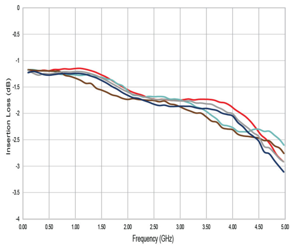
Figure 8. Insertion Loss vs. Frequency, All Paths
