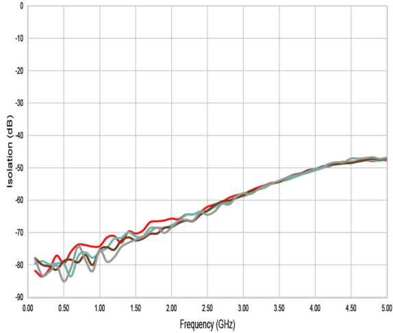
Figure 11. Isolation: RFX-RFX @ 3.0 V
