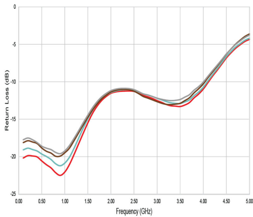
Figure 17. Return Loss: All Paths, Terminated
