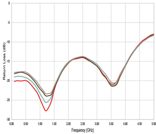
Figure 15. Return Loss: RFC @ 3.0 V
