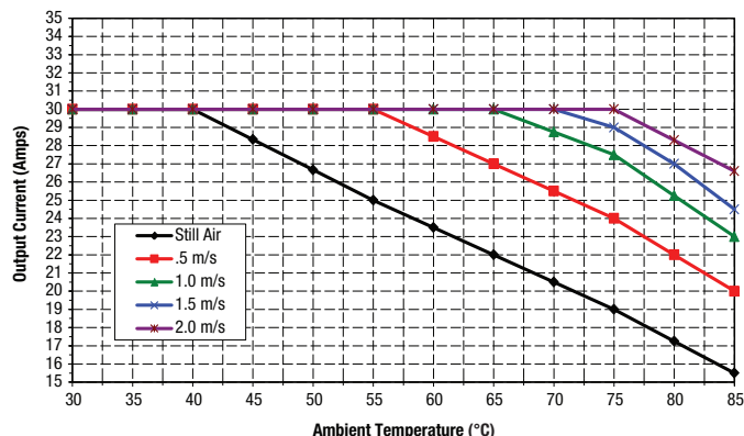
Temperature Derating @1Vout Vin 12V (air flow from Pin 13 (input) to Pin 1 (output) on PCB)
