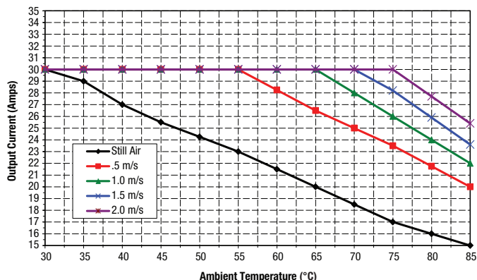
Temperature Derating @1.8Vout Vin 12V (air flow from Pin 13 to Pin 1 on PCB)
