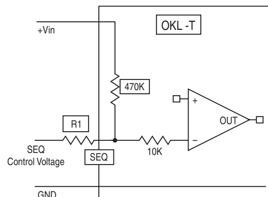
Figure 7. Sequencing Signal Interface of Module
