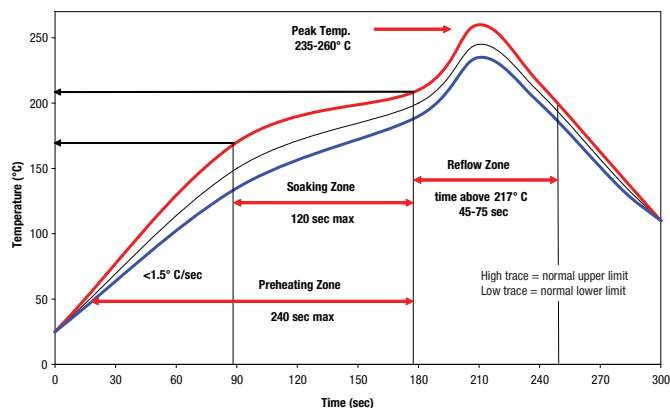
Recommended Lead-free Solder Reflow Profile
