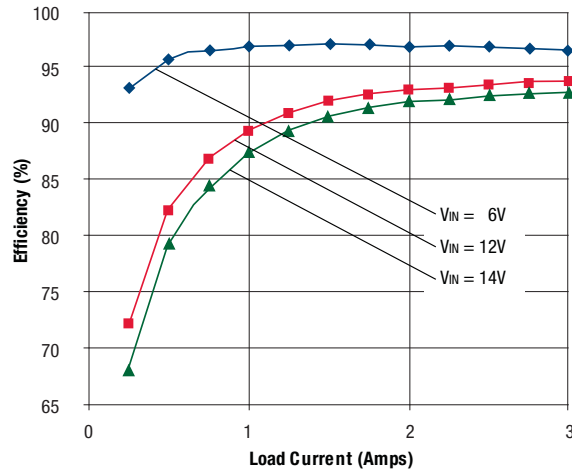
OKL-T/3-W12 Efficiency vs. Line Voltage and Load Current +25 °C (Vout = 5V)
