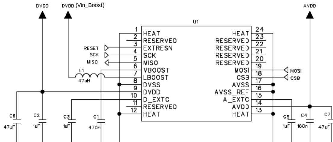
Figure 22. Application schematic.
