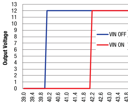
Output v. Input Voltage @ No Load
