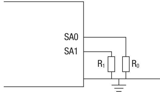
Figure 2. Schematic of Connection of Address Resistors
