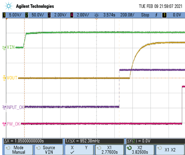
Figure 1: Turn-on by Vin; input to Input_OK signal; Back
