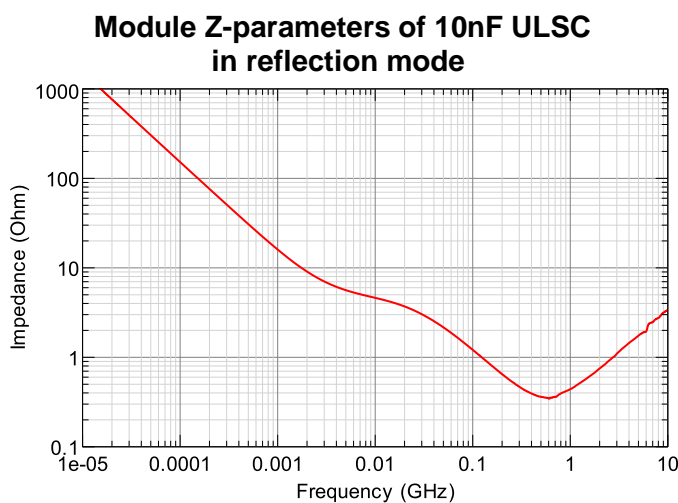
Figure 2 - 10nF ULSC measurement results (Impedance)
