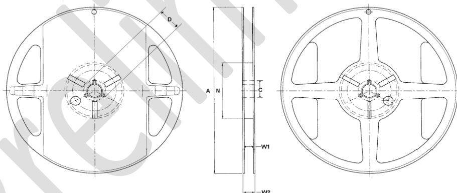
Figure 11 - Reel drawing
