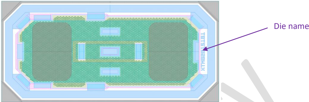
Figure 7 - Layout view
