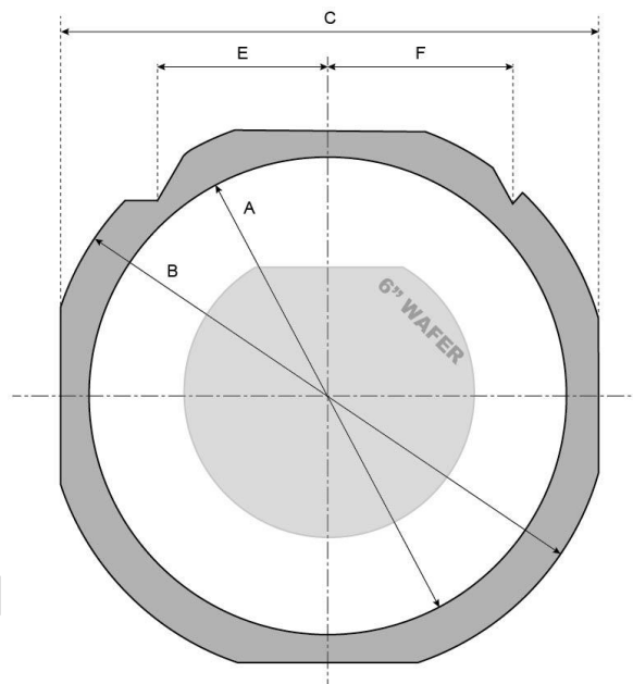
Figure 14 FF108 Frame with a 6" wafer
