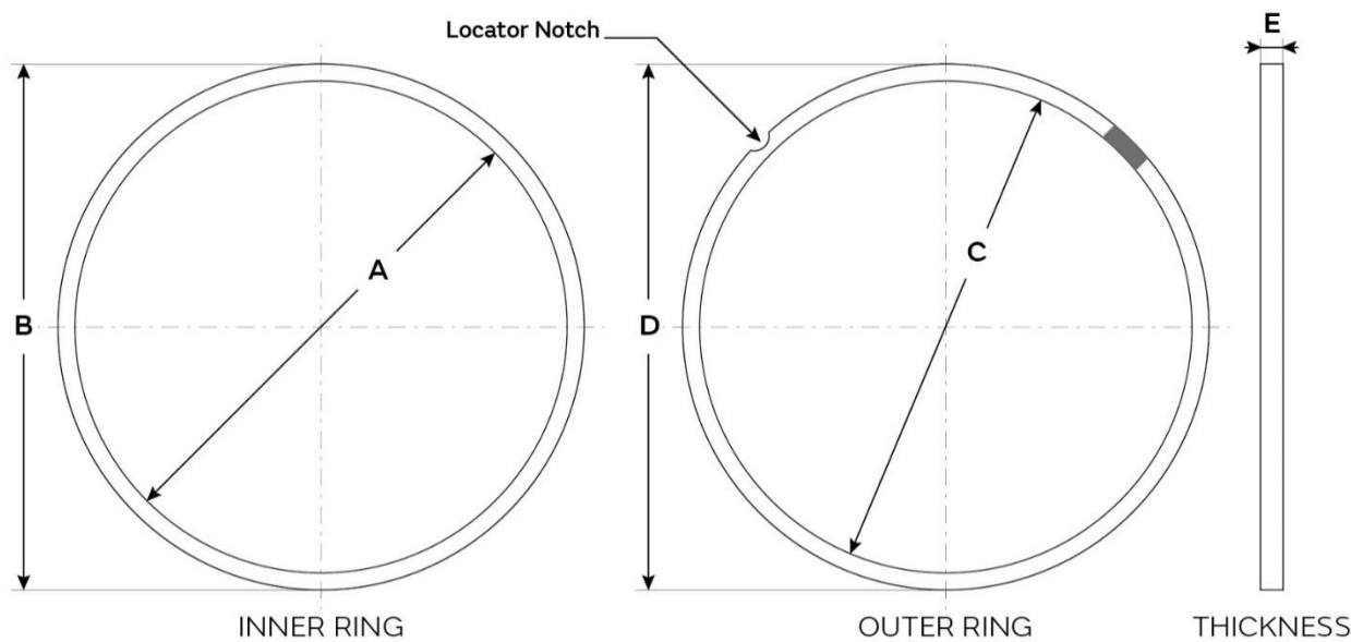
Figure 15 – Grip Ring drawing
