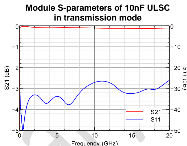
Figure 3 - 10nF ULSC measurement results (module of S-parameters)
