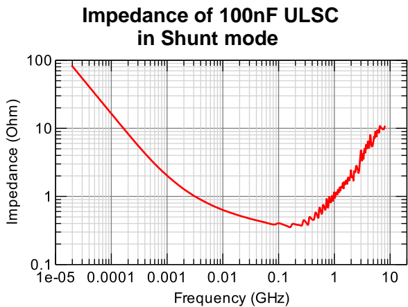
Figure 2 - 100nF ULSC Measured results (module of Z-parameters)
