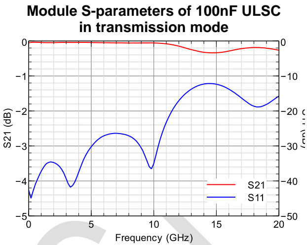
Figure 3 - 100nF ULSC measurement results (module of parameters)
