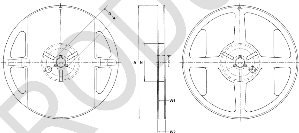
Figure 7 - Reel drawing
