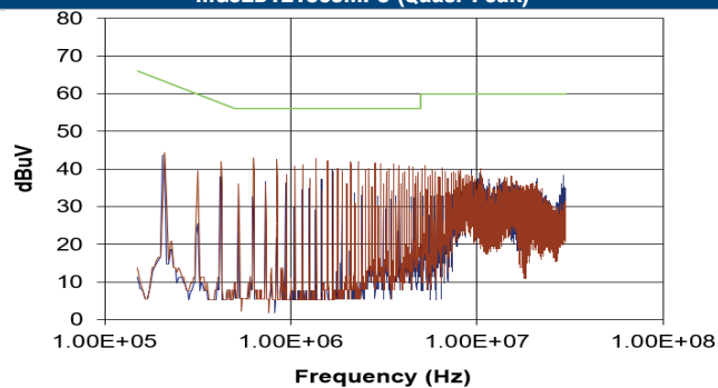
MGJ2D121509MPC (Quasi-Peak)
