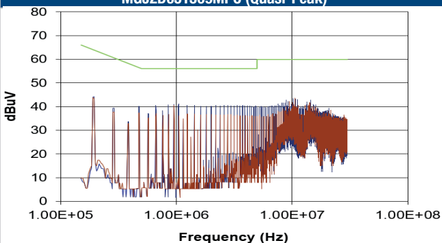
MGJ2D051509MPC (Quasi-Peak)
