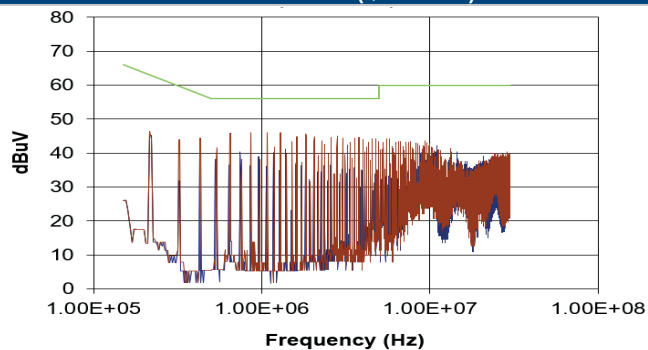
MGJ2D122005MPC (Quasi-Peak)
