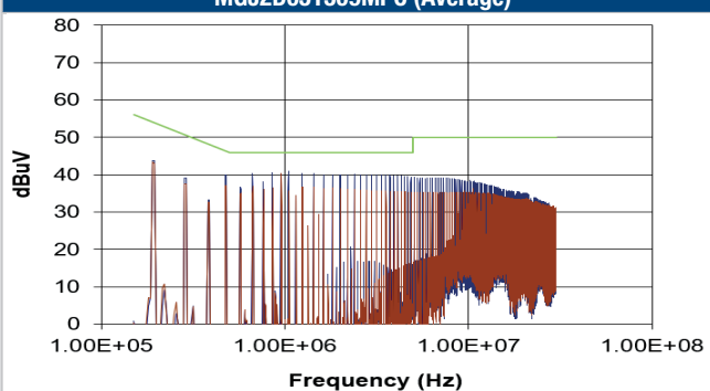
MGJ2D051509MPC (Average)
