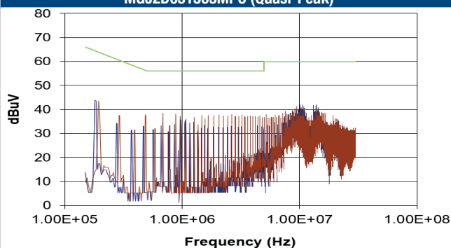
MGJ2D051505MPC (Quasi-Peak)
