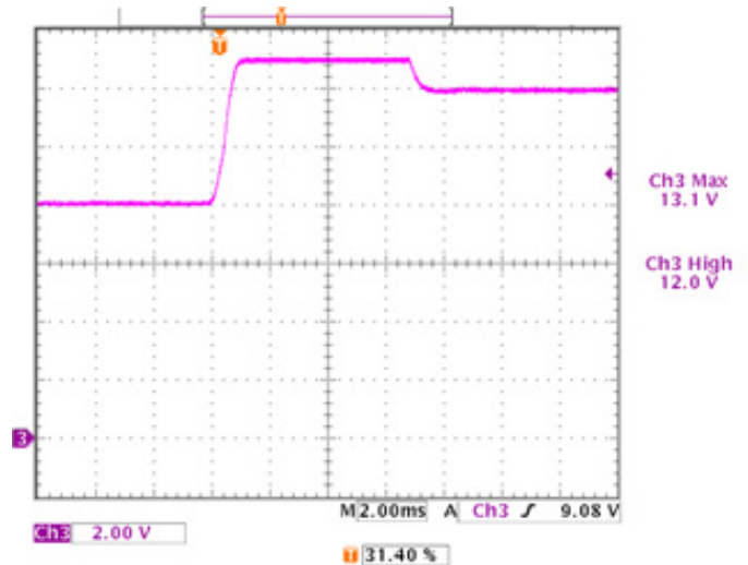
Typical Startup Waveform with a 8V bias voltage
