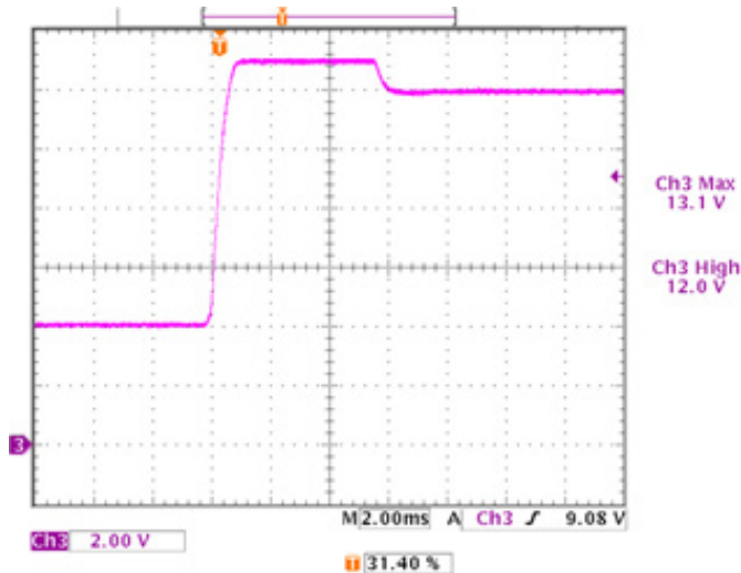
Typical Startup Waveform with a 4V bias voltage
