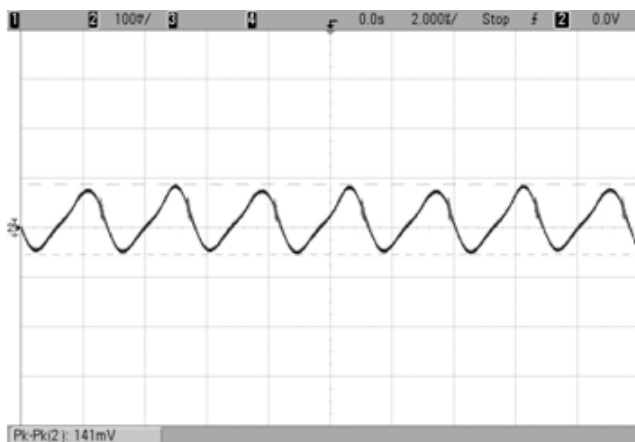
Output Ripple and Noise (Vin = 48V, Iout = 20A, Cload = 4700uF, Ta = +25°C)
