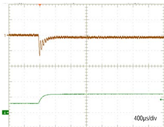
Transient Response (V in =48V, I out =3A to 6A, Ta=+25°C) Ch1=V out , 100mV/div, Ch4=I out , 5A/div
