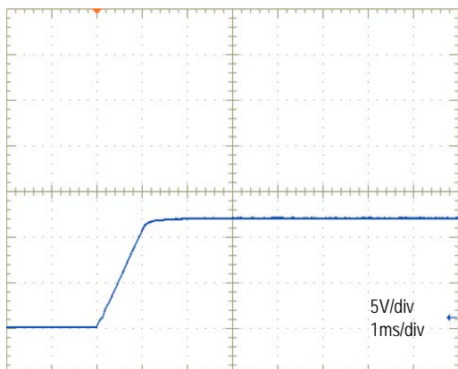
V out Start-up (V in =48V, I out =6A, Ta=+25°C)
