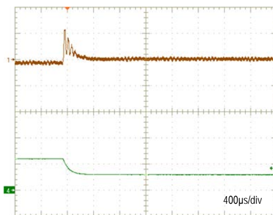
Transient Response (V in =48V, I out =6A to 3A, Ta=+25°C) Ch1=V out , 100mV/div, Ch4=I out , 5A/div
