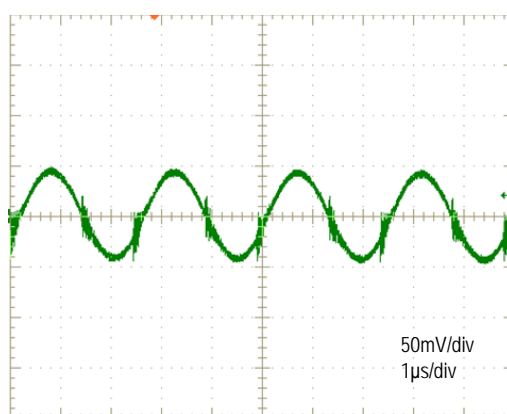
Output Ripple and Noise (V in =48V, I out =6A, Ta=+25°C)
