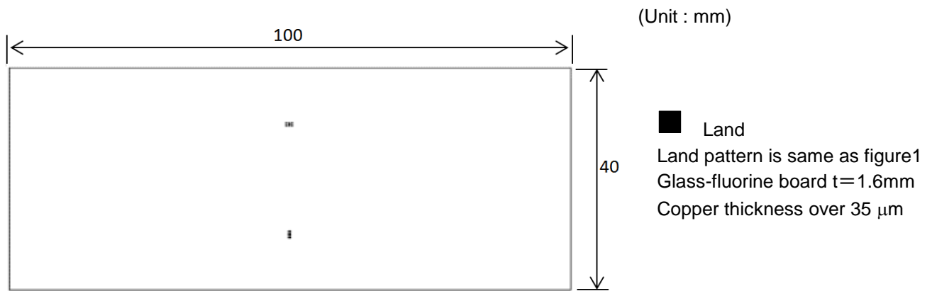
Fig. 2 Testing board
