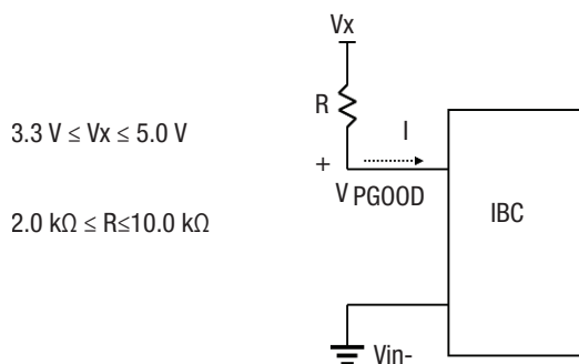
Figure 3. External circuit configuration for PGOOD signal
