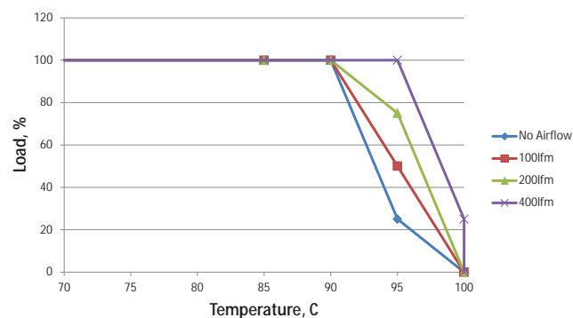
MTC1S2405MC- 18Vin
