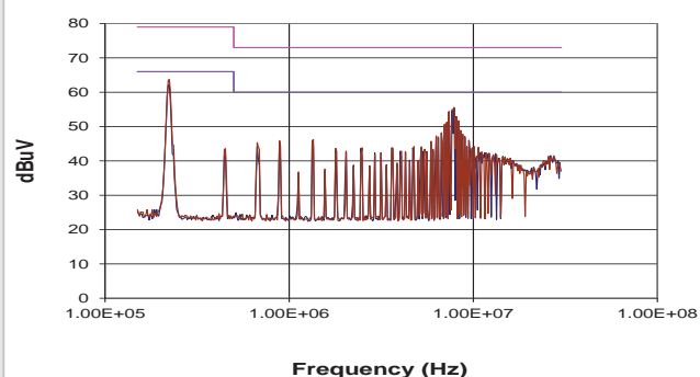
MTC1S2405MC
