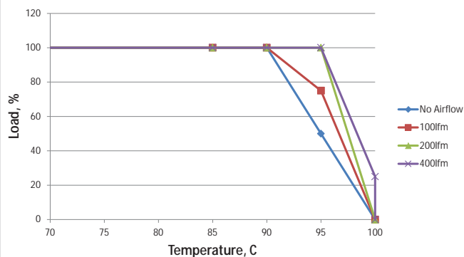
MTC1S2403MC- 18Vin
