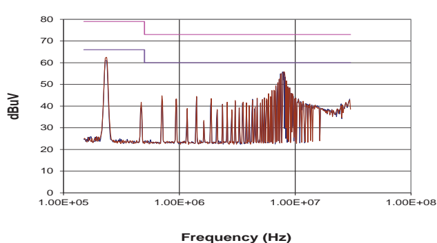
MTC1S2412MC
