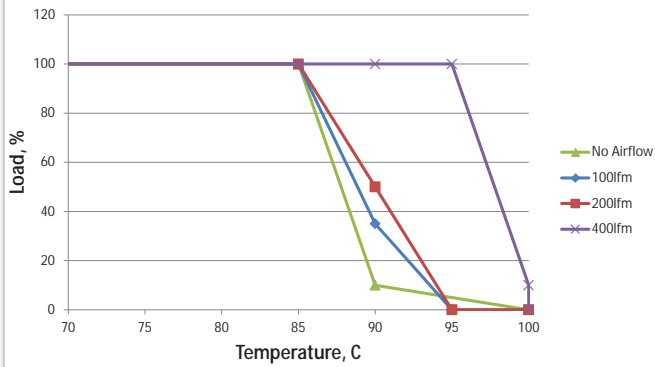
MTC1S1212MC- 18Vin
