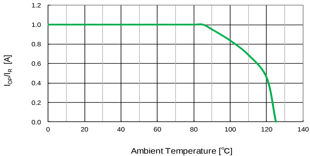
Current Derating Curve
