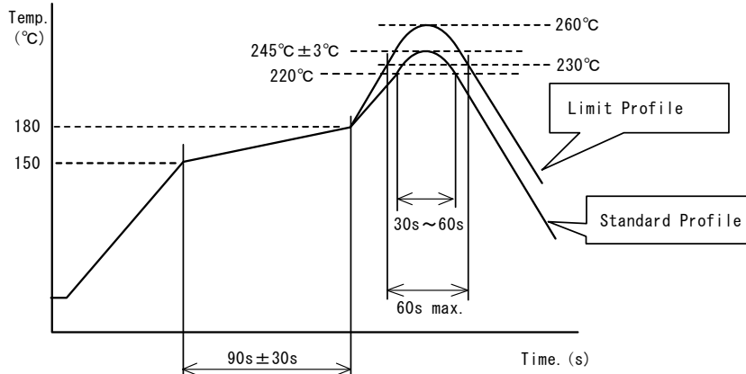
Soldering profile
