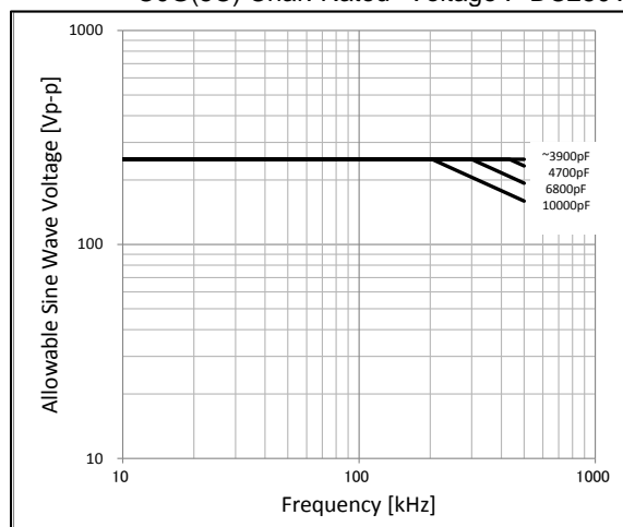
C0G(5C) Char. Rated Voltage : DC250V
